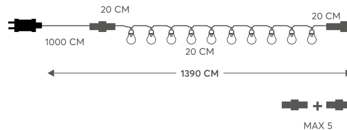
20 LED BULBS WITH BALLS DECORATIONS "PARTY GARLAND"
