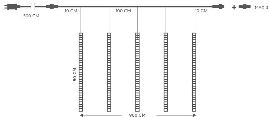
SERIES 5 TUBES OF 50 CM, 240 WHITE LED
