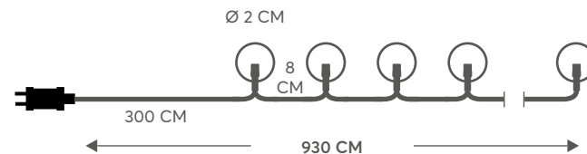
GARLAND WITH 80 WARM WHITE BULB LED AND BALLS DECORATIONS
