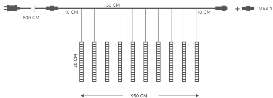
SERIES 10 TUBES OF 20 CM, 240 WHITE LED
